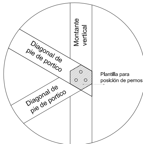
DETALLE A vista interior
